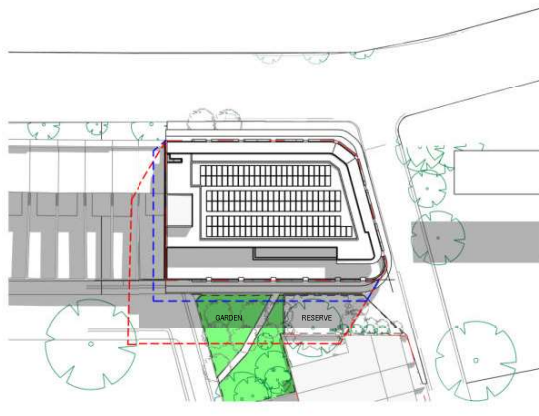
2 Shadows (Equinox)-21 March 9.30am 1:500
