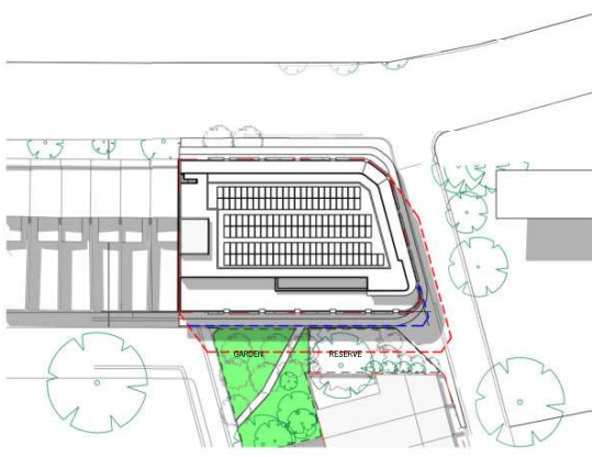
8 Shadows (Equinox)-21 March 12.30pm 1:500
